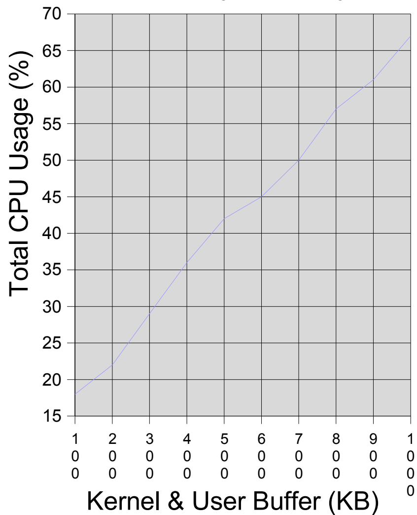
MinToCopy: 60 Bytes
